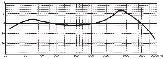
QKICK Frequency Chart
