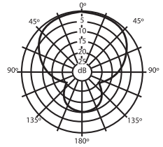
QKICK Polar Pattern
