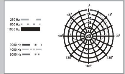
Q8 pickup pattern
