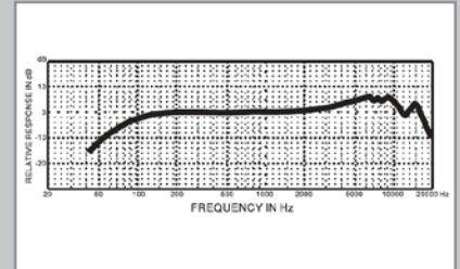
Q8 frequency chart
